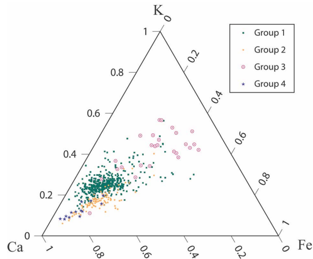
Figure 3. Ca-K-Fe triangular diagram for all the clay tablet using the data for Ca, K, and Fe in Appendix.
