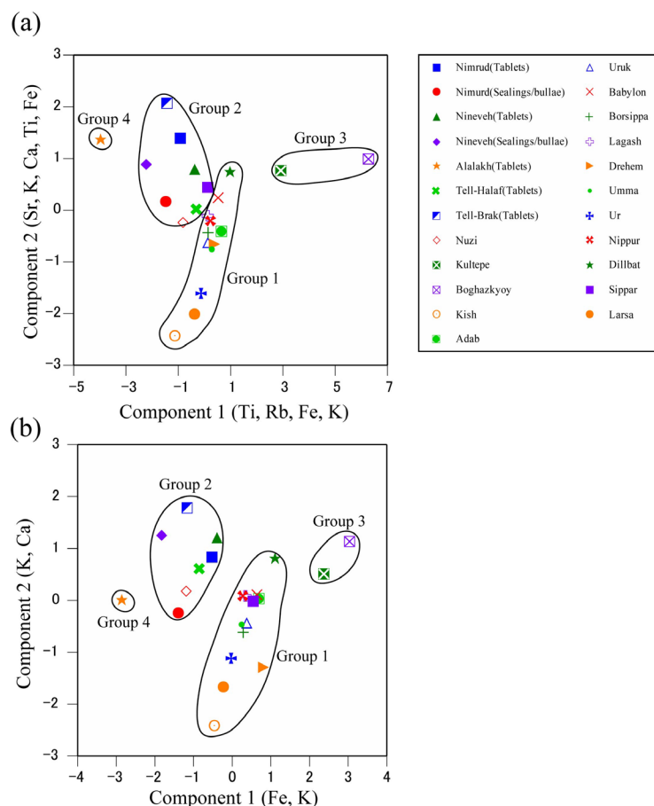
Figure 2. Results of the principal component analysis of the clay tablets. (a) Results using the averaged data for Ca, K, Fe, Ti, Rb, and Sr in Table 2 ; (b) results using the averaged data for Ca, K, and Fe, in Table 2 . Group 1 corresponds to the lower stream area of the Tigris and Euphrates River, Group 2 corresponds to the upper stream area of the Tigris and Euphrates River, Group 3 corresponds to the northern and central areas (Boghazkyoy and Kultepe) in Turkey, and Group 4 corresponds to the southern area (Alalakh) in Turkey.
