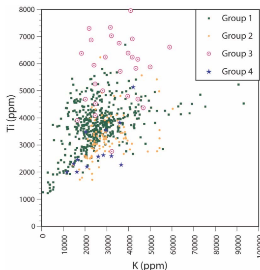
Figure 6. Ti-K diagram for all the clay tablets based on the grouping obtained by the principal component analysis (Figure 2) and the cluster analysis (Figure 4) using the data in Appendix. The four groups were distinguished with some overlap.
